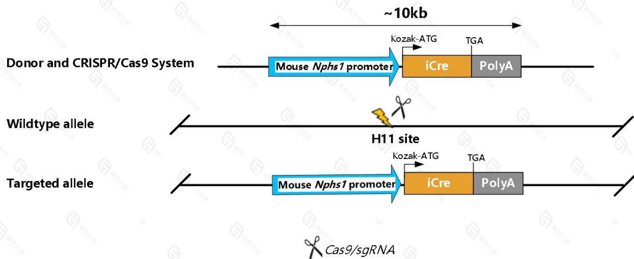
Fig.1 Schematic diagram of C57BL/6JGpt-H11-Nphs1-iCre model strategy.
